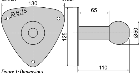
Figure 1: Dimensions
