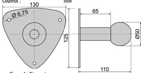
Figure 1 : Dimensions
